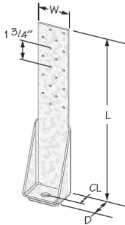
HTT16/HTT22 similar
