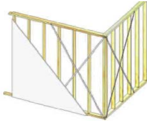
Typical RWB, WB installation
