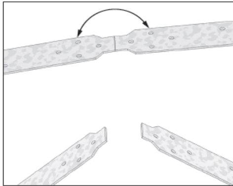
RWB pre-embossed snap-off points
